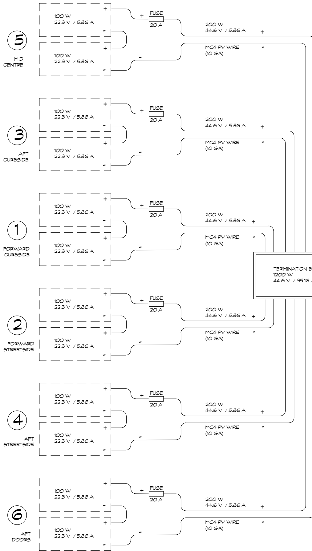
2 SOLAR SYSTEM - WIRING DIAGRAM A-FP11a NOT TO SCALE
